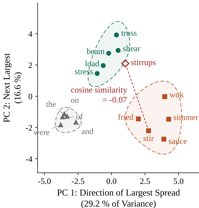
After Training (GloVe Word Vectors)
